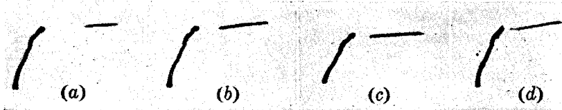
FIG. 8-36.—Steady-state characteristics showing the effect of changing the pulser impedance on the minimum current that can be drawn. (a) No series resistor; (b) 200 ohms in series; (c) 500 ohms in series; (d) 1000 ohms in series.
